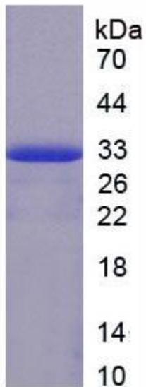
SDS-PAGE Image
