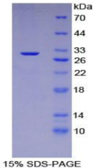
Figure. SDS-PAGE
