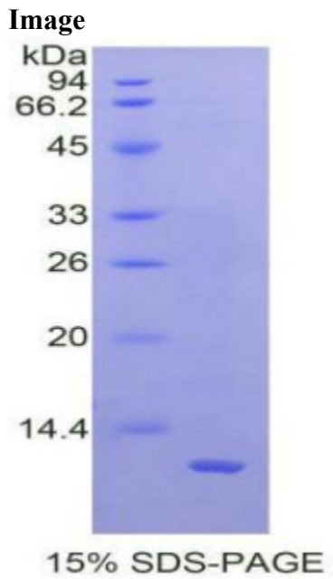
SDS-PAGE Image
