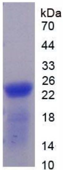
SDS-PAGE Image
