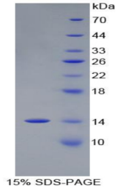
Figure. SDS-PAGE
