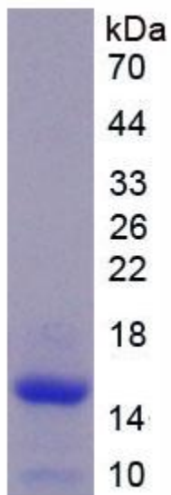
SDS-PAGE Image
