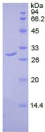
SDS-PAGE Image
