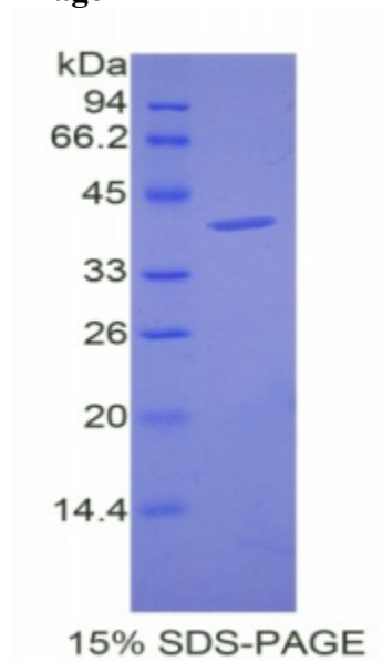
SDS-PAGE Image
