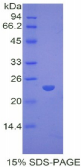
SDS-PAGE Image
