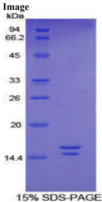
SDS-PAGE Image
