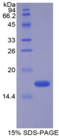
SDS-PAGE Image
