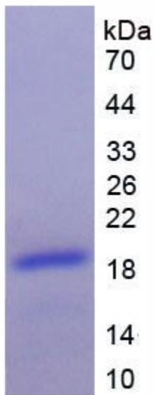
SDS-PAGE Image
