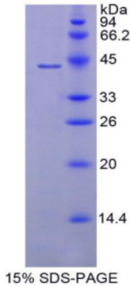
SDS-PAGE Image
