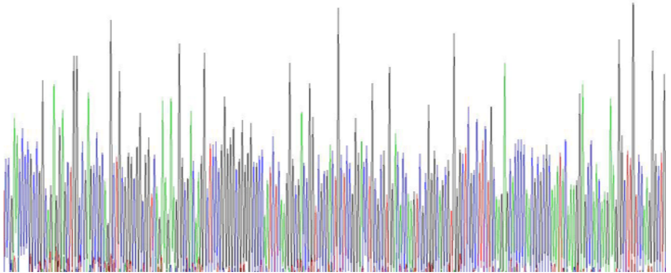
SDS-PAGE Image
