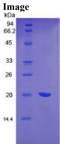
Figure. SDS-PAGE
