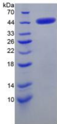
Figure. SDS-PAGE
