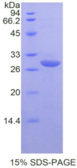
SDS-PAGE Image
