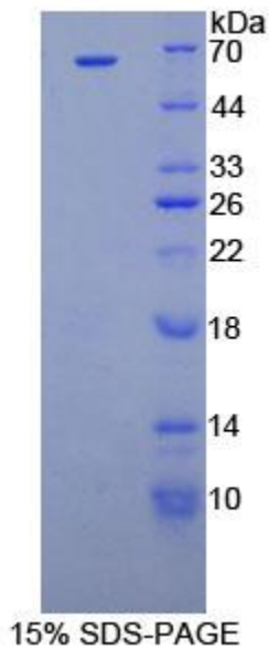
SDS-PAGE Image
