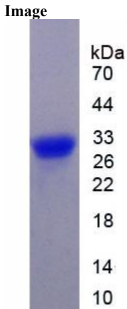
Figure. SDS-PAGE
