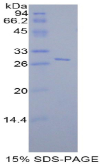
SDS-PAGE Image
