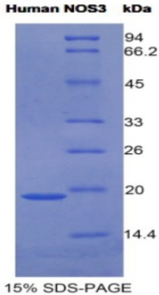
Figure. SDS-PAGE
