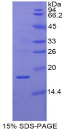
SDS-PAGE Image
