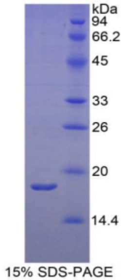
SDS-PAGE Image
