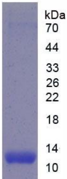
SDS-PAGE Image
