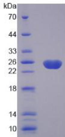
SDS-PAGE Image
