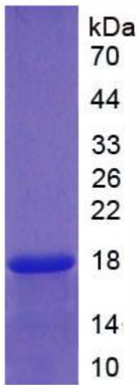
SDS-PAGE Image
