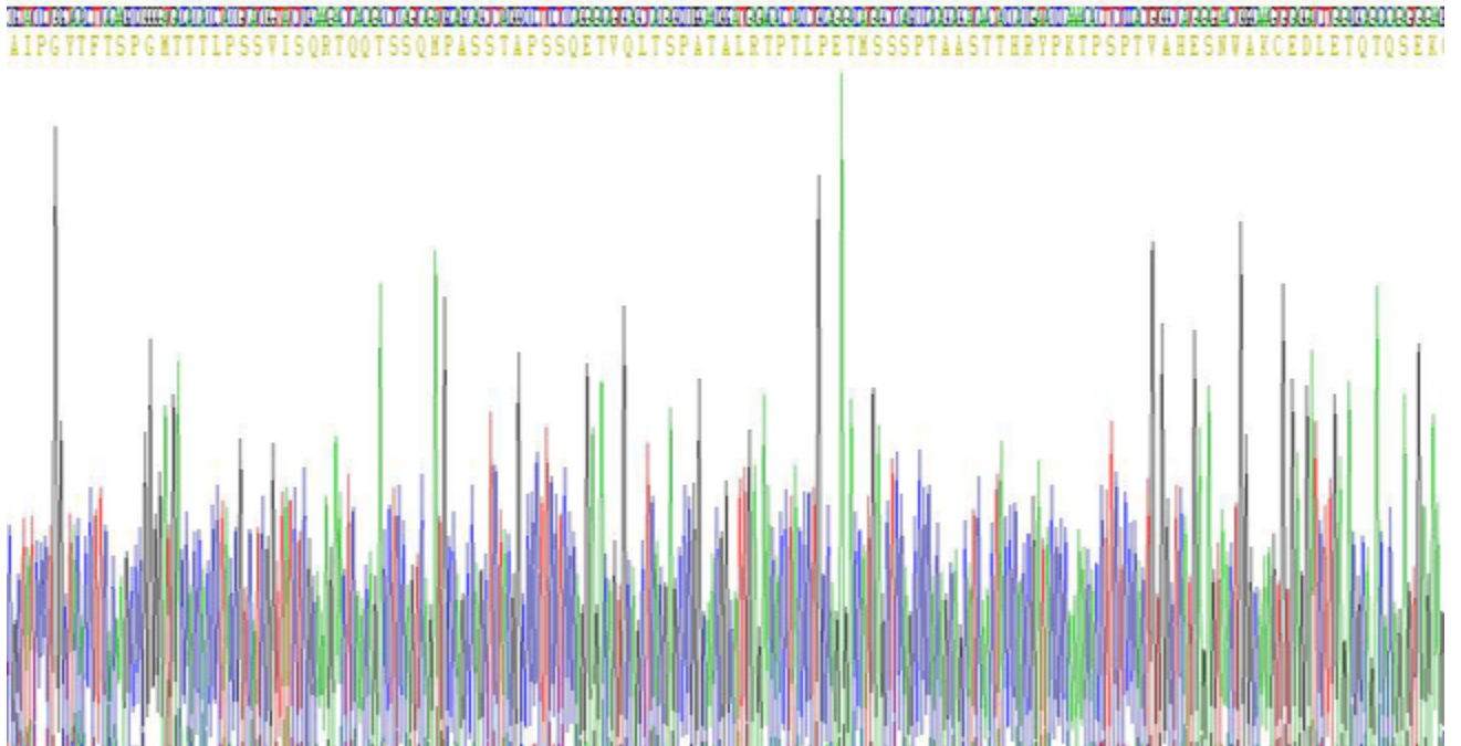
SDS-PAGE Image
