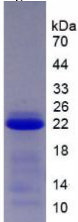
SDS-PAGE Image
