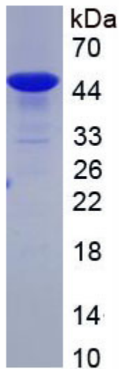
Figure. SDS-PAGE
