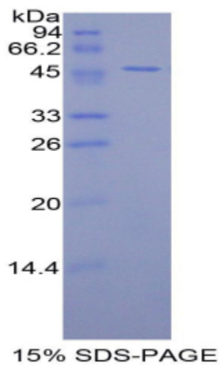
SDS-PAGE Image
