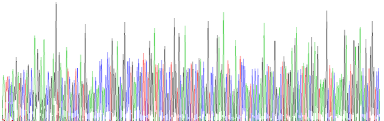
Figure. SDS-PAGE
