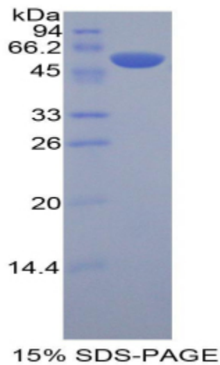
SDS-PAGE Image
