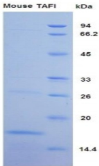
SDS-PAGE Image
