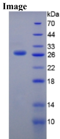
Figure. SDS-PAGE
