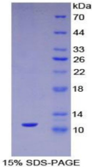
Figure. SDS-PAGE
