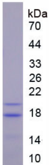
Figure. SDS-PAGE
