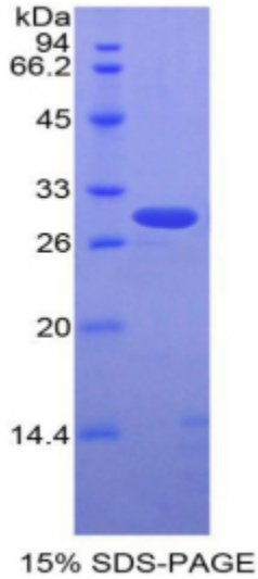
SDS-PAGE Image
