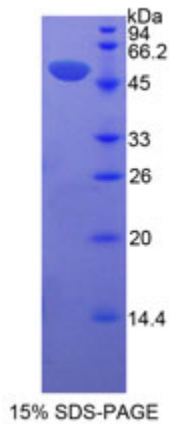
SDS-PAGE Image
