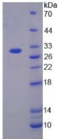
SDS-PAGE Image
