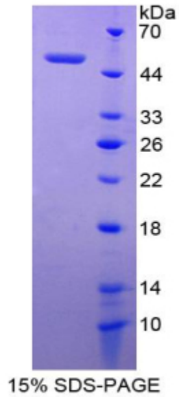
SDS-PAGE Image
