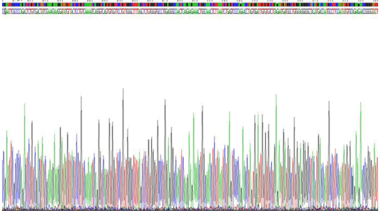
Figure. SDS-PAGE
