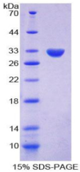
SDS-PAGE Image
