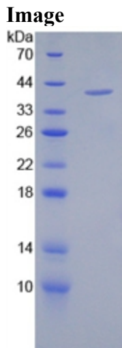
Figure. SDS-PAGE
