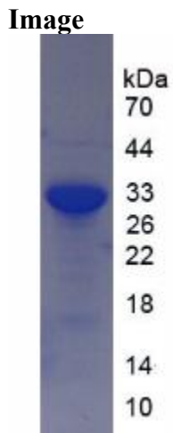
Figure. SDS-PAGE
