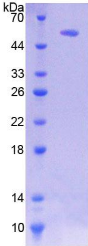
SDS-PAGE Image
