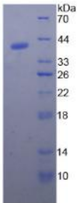
SDS-PAGE Image
