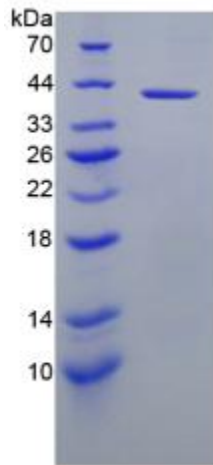
SDS-PAGE Image
