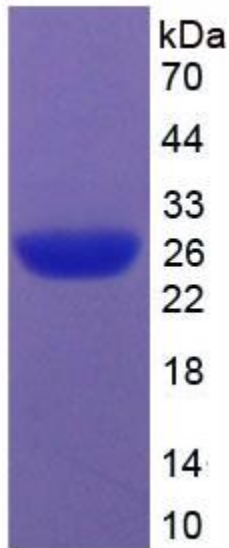
SDS-PAGE Image
