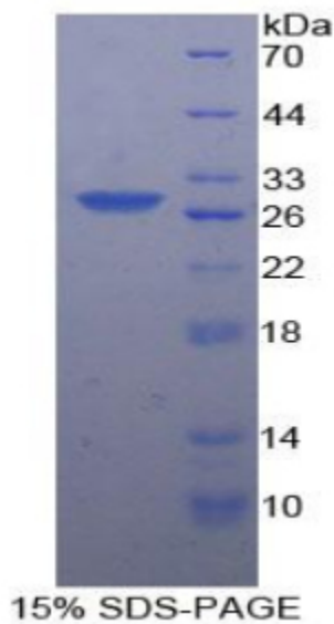
Figure. SDS-PAGE
