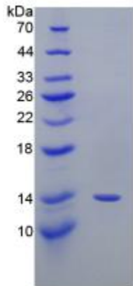
Figure. SDS-PAGE
